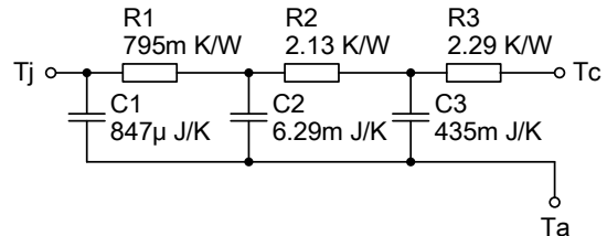
Figure 5. Example of thermal model: Cauer RC thermal circuit network Diode manufactured by ROHM: RB085T-40NZ
