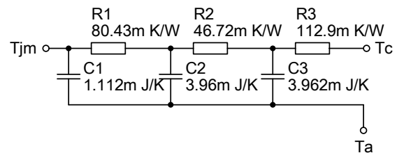
Figure 5. Example of thermal model: Cauer RC thermal circuit network IGBT manufactured by ROHM: RGT VX6TS65D
