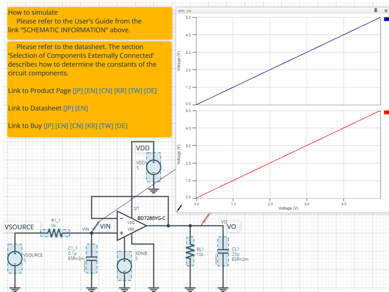
Figure 1. Simulation Schematic
