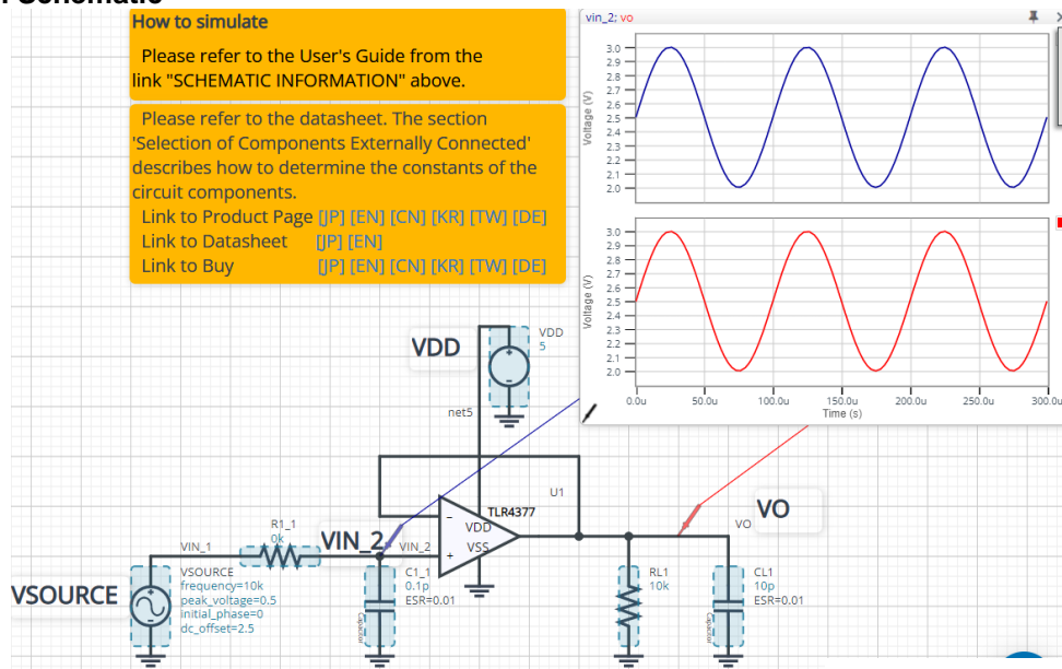
Figure 1. Simulation Schematic
