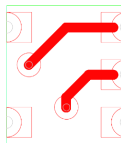
Figure 4. Layout (Bottom View)
