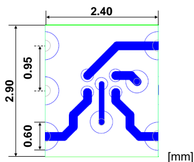
Figure 3. Layout (Top View)
