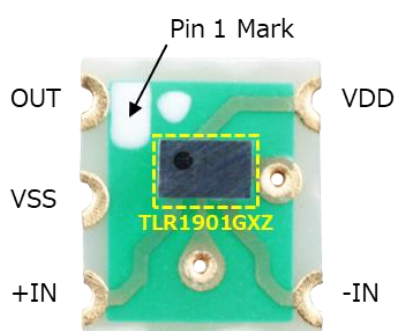
Figure 1. Outline and Pin Configuration (Top View)
