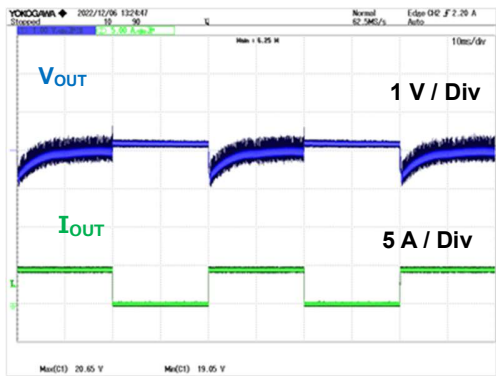
Figure 19. V_{IN} = 90 Vac, I_{OUT} = switch 0 A / 4.5 A
