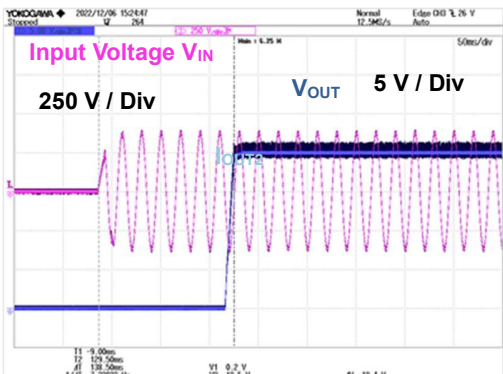
Figure 18. V_{IN} = 264 Vac, I_{OUT} = 4.5 A
