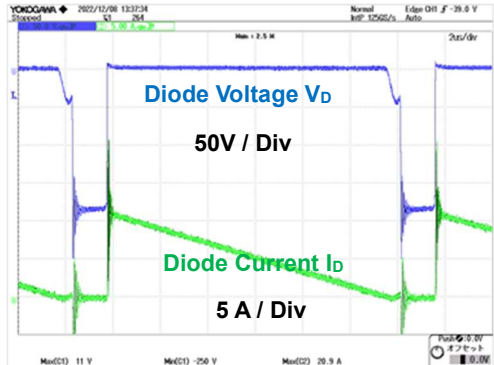
Figure 14. Diode Wave Form V_{IN} = 264\text{Vac} , I_{OUT1} = 4.5\text{A}
