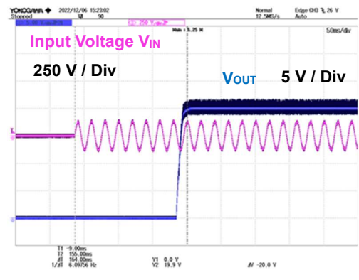
Figure 17. V_{IN} = 90 Vac, I_{OUT} = 4.5 A
