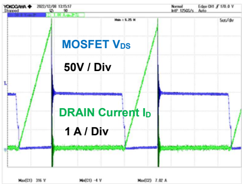
Figure 11. MOSFET Wave Form V_{IN} = 90 \text{ Vac} , I_{OUT}=4.5\text{A}
