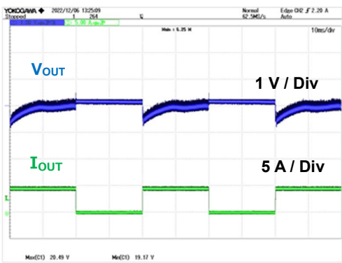
Figure 20. V_{IN} = 264 Vac, I_{OUT} = switch 0A / 4.5 A
