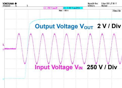
Figure 18. V_{IN} = 264 \text{ Vac} , I_{OUT} = 2A
