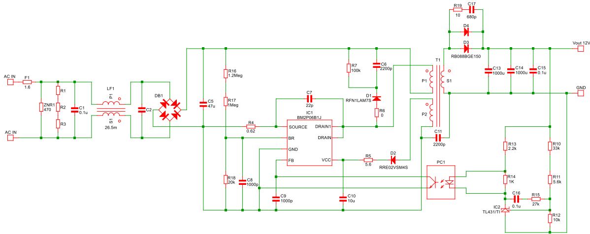
Figure 25. BM2P06B1J-EVK-001 Schematics
