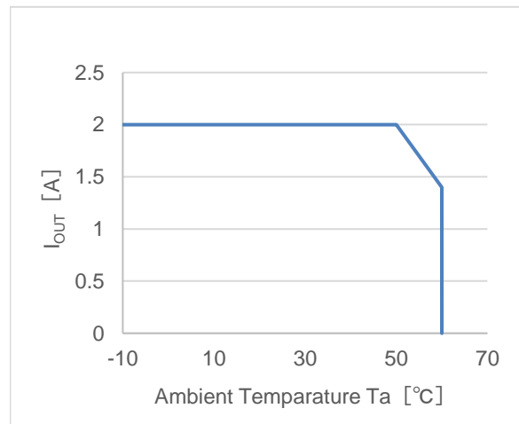
Figure 2. Temperature derating curve
