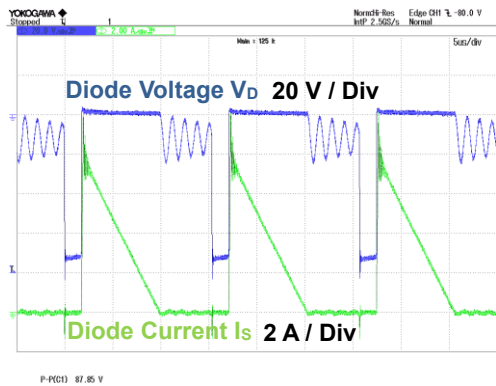
Figure 14. V_D , I_S V_{IN} = 264 Vac, I_{OUT} = 2 A
