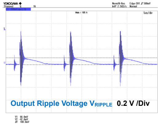
Figure 22. V_{IN} = 264 \text{ Vac} , I_{OUT} = 2 \text{ A}
