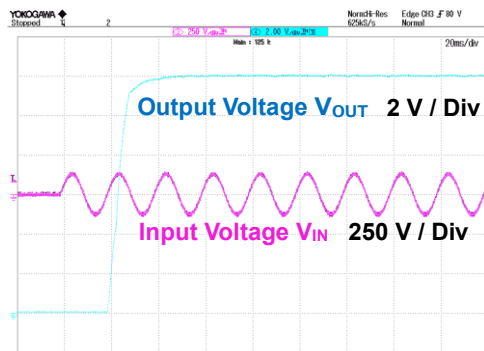
Figure 17. V_{IN} = 90 \text{ Vac} , I_{OUT} = 2A
