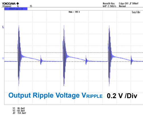
Figure 21. V_{IN} = 90 \text{ Vac} , I_{OUT} = 2 \text{ A}
