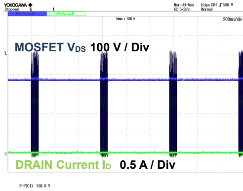
Figure 15. V_{DS} , I_D V_{IN} = 264 \text{ Vac} , V_{OUT} Shorted
