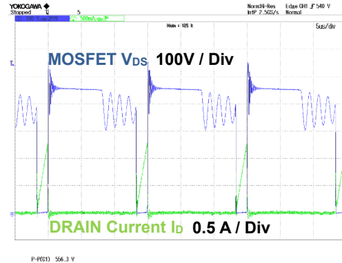
Figure 12. V_{DS} , I_D V_{IN} = 264 Vac, I_{OUT} = 2 A
