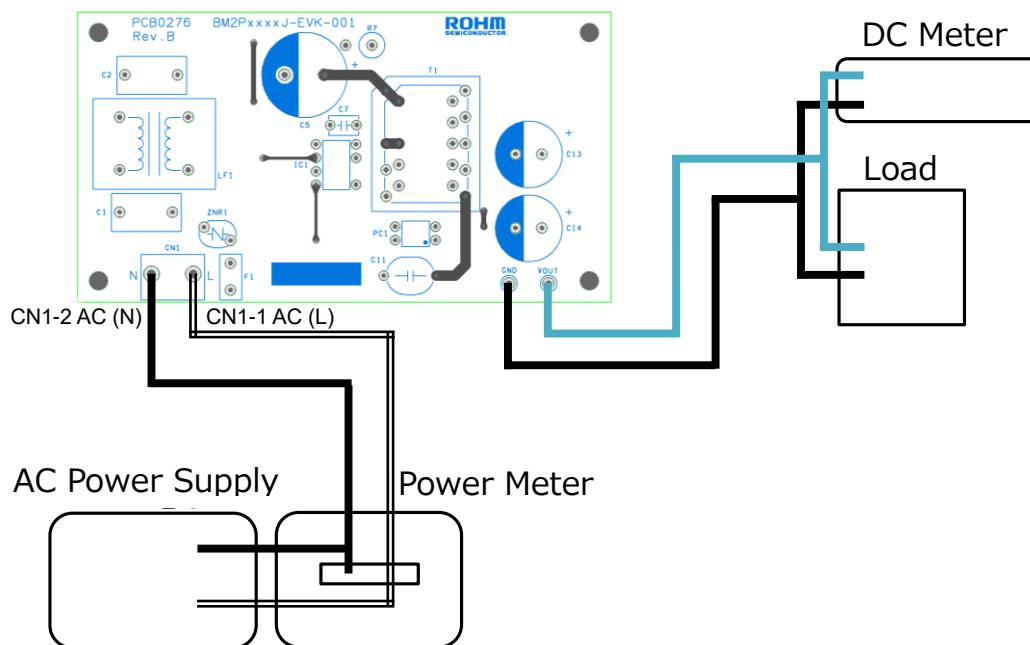
Figure 3. Diagram of How to Connect
