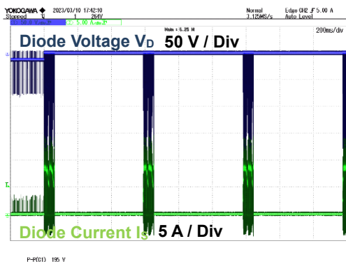
Figure 16. V_D , I_S VIN = 264 Vac, V_{OUT} Shorted
