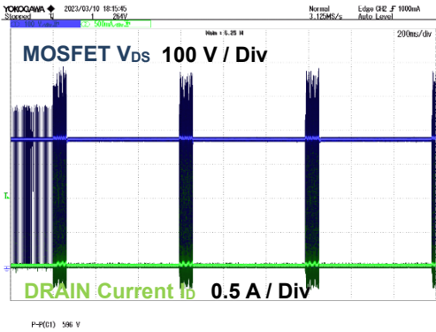
Figure 15. V_{DS} , I_D VIN = 264 Vac, V_{OUT} Shorted
