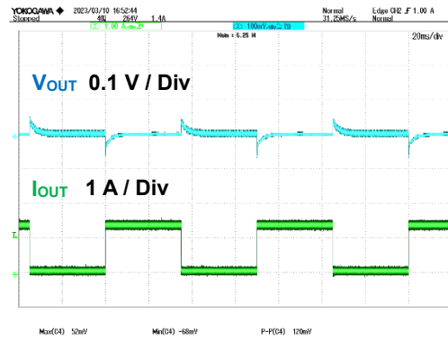
Figure 20. V_{IN} = 264 \text{ Vac} , I_{OUT} = \text{switch } 0.06 \text{ A} / 1.4 \text{ A}
