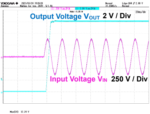
Figure 18. V_{IN} = 264 Vac, I_{OUT} = 1.4A
