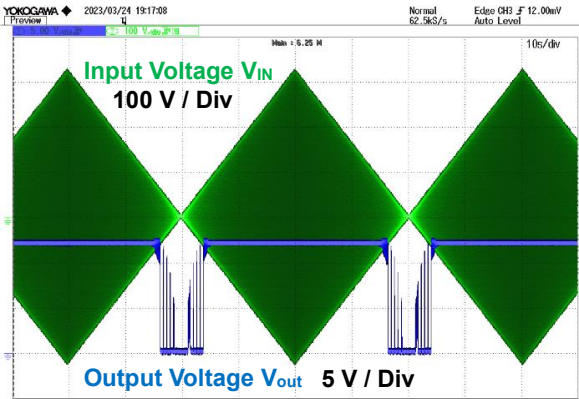
Figure 10. V_{IN} 0 V to 230 V
