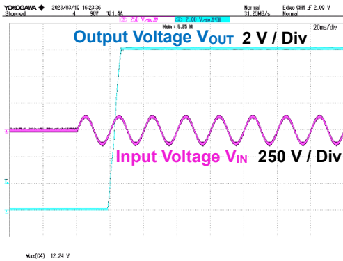
Figure 17. V_{IN} = 90 Vac, I_{OUT} = 1.4A
