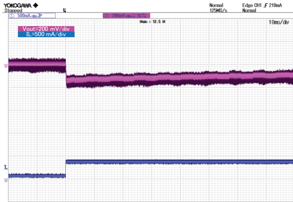
Figure 23. Iout and Vout (5 MHz Filter) VIN = 264 Vac, IOU T = 0.05 A to 0.35 A
