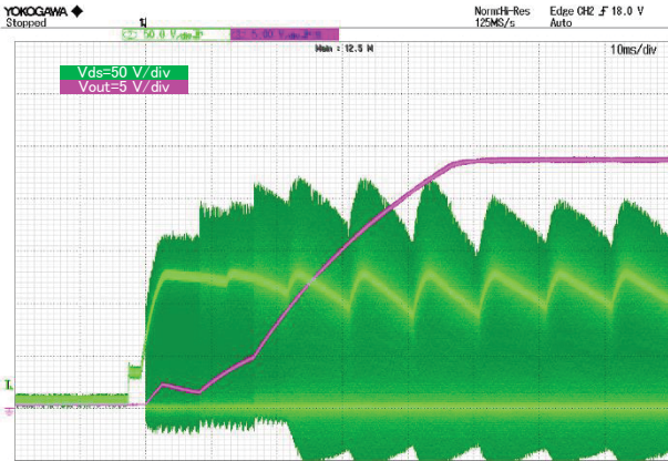
Figure 20. Vds and Vout VIN = 90 Vac, IOUt = 0.35 A
