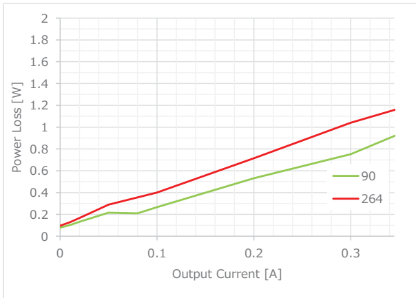
Figure 10. IOU T vs. Power
