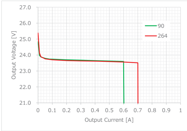
Figure 8. IOU T vs. V OUT
