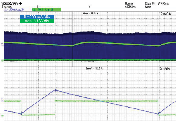
Figure 16. Vds and IL VIN = 90 Vac, IOUt = 0.35 A
