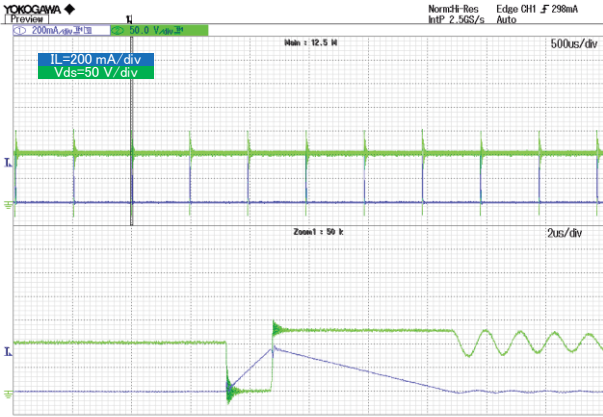
Figure 12 Vds and IL VIN = 90 Vac, IOUt = 0 A
