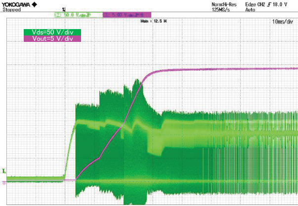
Figure 18. Vds and Vout VIN = 90 Vac, IOUt = 0 A
