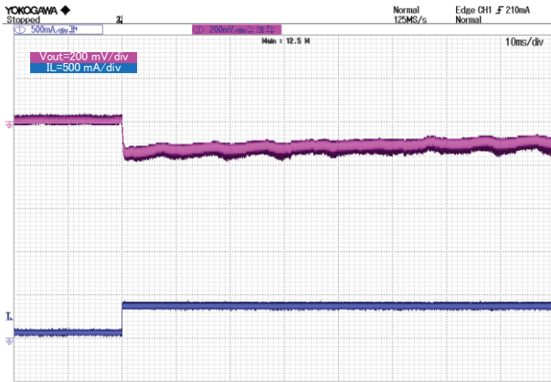
Figure 22. Iout and Vout (5 MHz Filter) VIN = 90 Vac, IOU T = 0.05 A to 0.35 A
