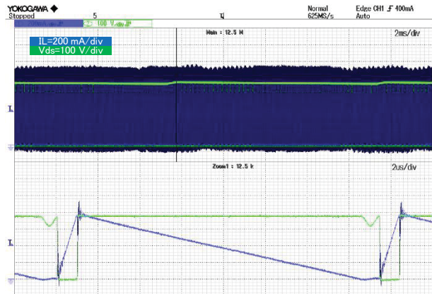
Figure 17. Vds and IL VIN = 264 Vac, IOUt = 0.35 A
