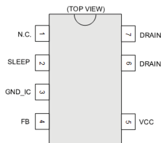
Figure 7. Pin Configuration
