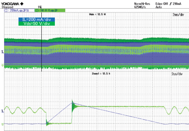
Figure 14. Vds and IL VIN = 90 Vac, IOUt = 0.2 A
