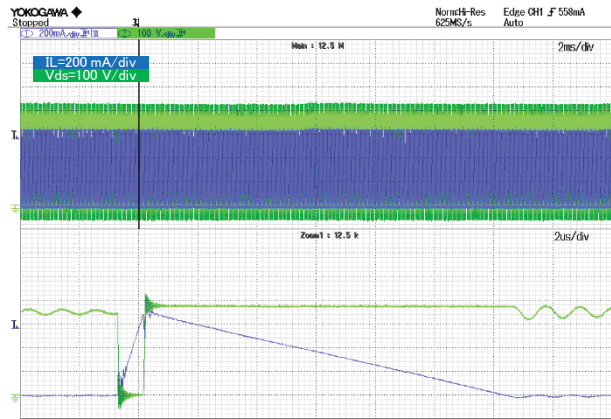
Figure 15. Vds and IL VIN = 264 Vac, IOUt = 0.2 A
