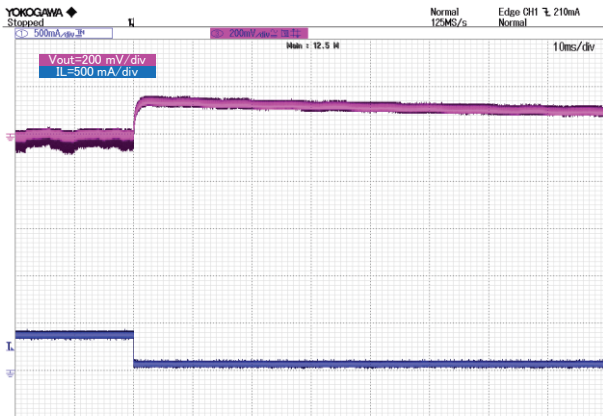
Figure 24. Iout and Vout (5 MHz Filter) VIN = 90 Vac, IOU T = 0.35 A to 0.05 A
