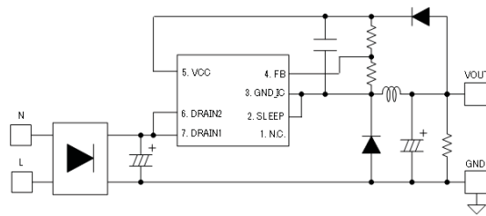
Figure 2. BM2PDA1Y-EVK-001 Simple Schematic
