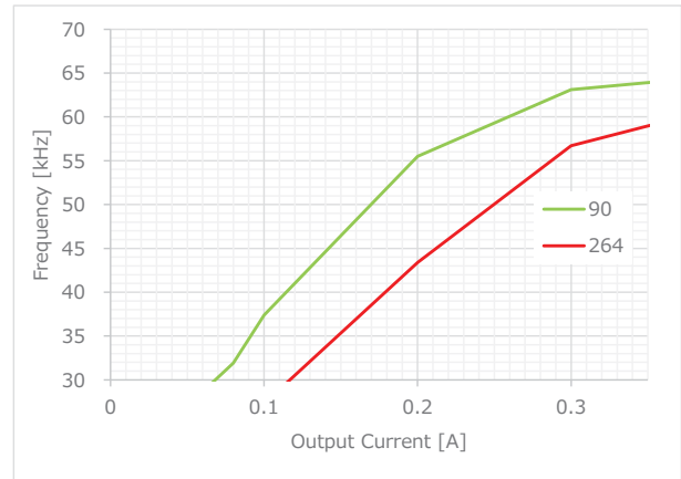
Figure 11. IOU T vs. Frequency
