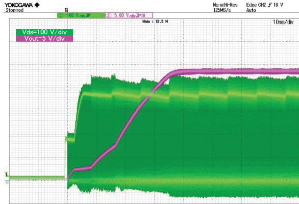
Figure 21. Vds and Vout VIN = 264 Vac, IOUt = 0.35 A
