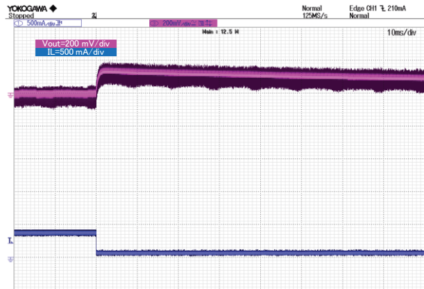
Figure 25. Iout and Vout (5 MHz Filter) VIN = 264 Vac, IOU T = 0.35 A to 0.05 A
