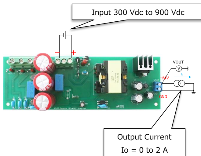
Figure 3. Input with DC power supply
