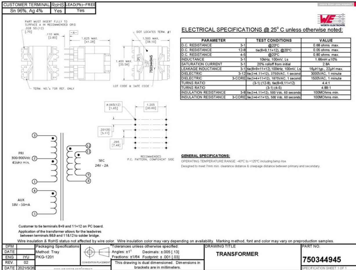
Figure 5. Transformer Specification
