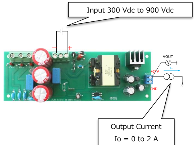
Figure 3. Input with DC power supply
