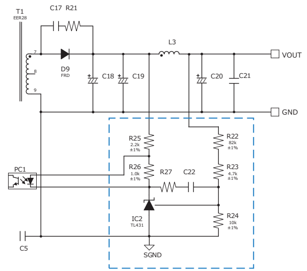
Figure 21. Feed-back Circuit
