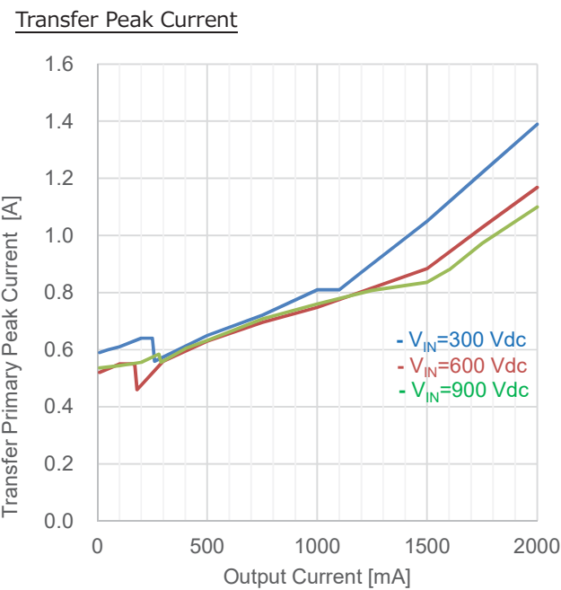
Figure 30. Transfer Primary Peak Current ( I_{OUT} vs I_{PPK} )
