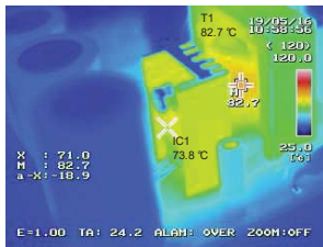
Figure 50-1. Thermal Image
