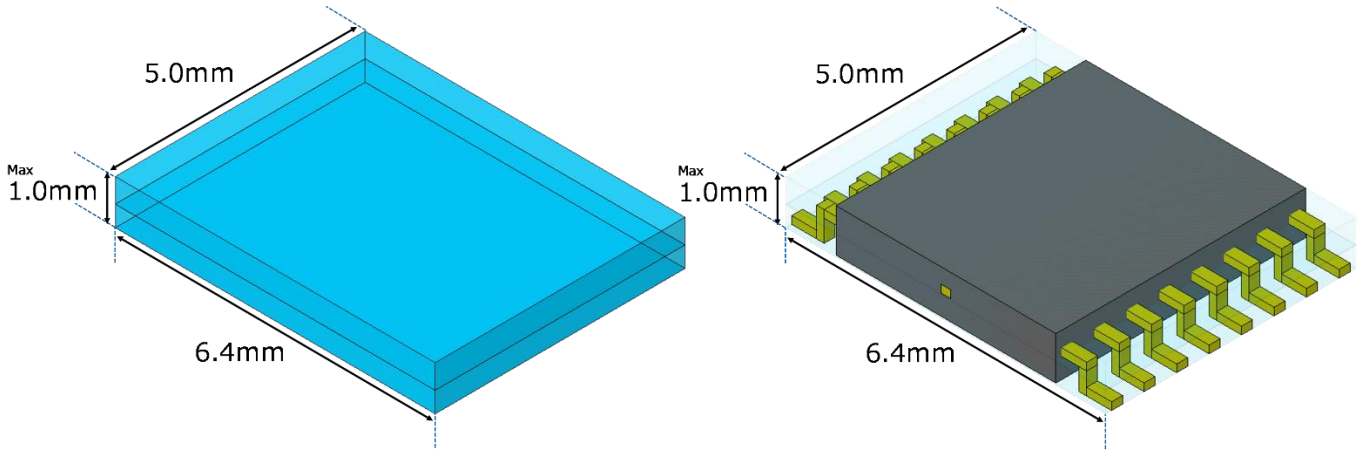
Figure 1. BD18347EFV-M Two-Resistor Thermal Model
