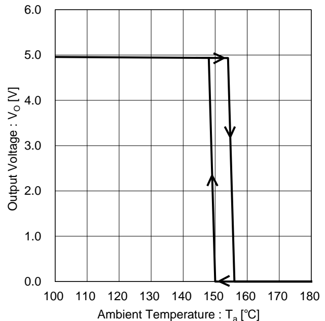
Figure 17-1. Thermal shutdown characteristics
