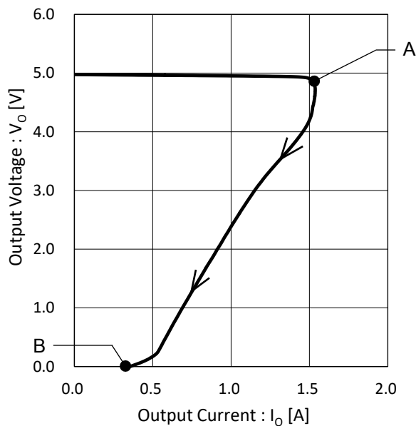
Figure 16-1. Characteristics of over current protection
