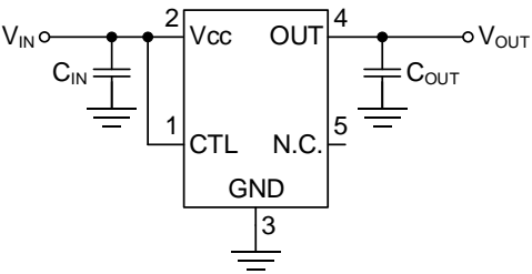
Figure 1-6. When not using the output ON/OFF function
