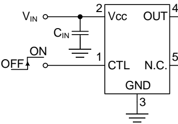
Figure 1-5. When using the output ON/OFF function
