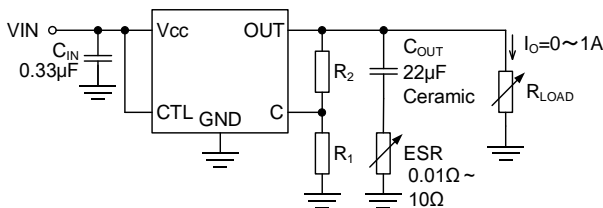
Figure 7-2. ESR stable operating range evaluation circuit
