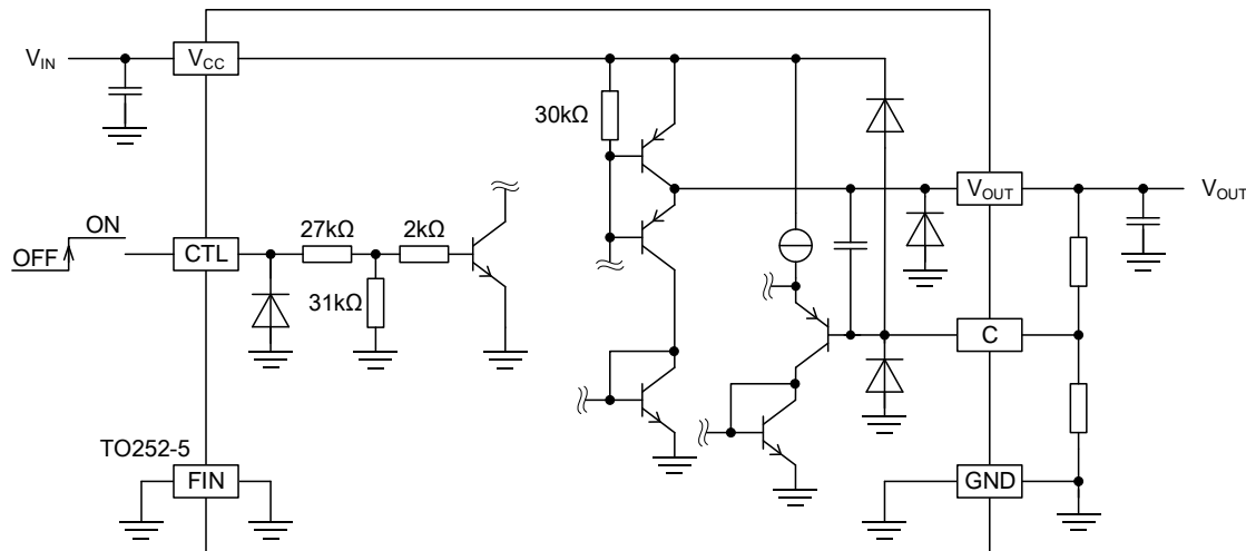
Figure 18-1. Adjustable output type equivalent circuit
