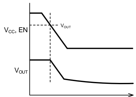
Figure 15-7. When V_{CC} and EN turn off gradually
