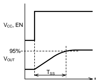
Figure 14-7. When V_{CC} and EN turns on abruptly
