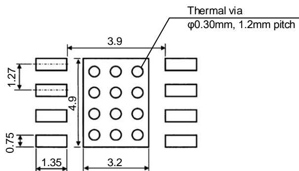
Figure 11-12. Footprint
