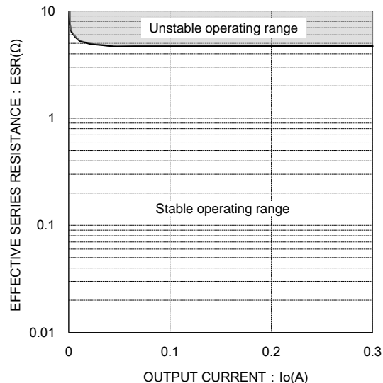
Figure 7-1. ESR stable operating range
