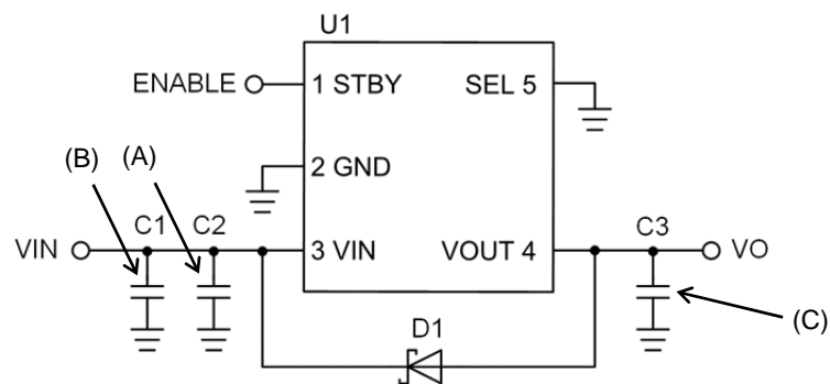
Figure 3. Circuit Diagram (SEL = Low)
