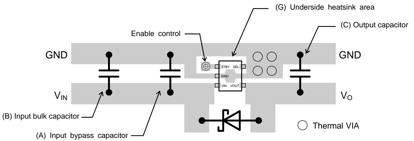
Figure 1. PCB Layout (SEL = Low)
