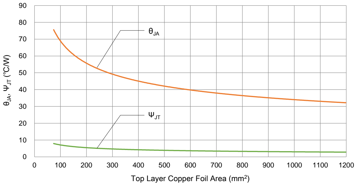
Figure 14. \theta_{JA} , \psi_{JT} vs. copper foil surface area
