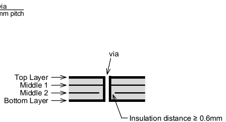
Figure 13. 4 layer board sectional view
