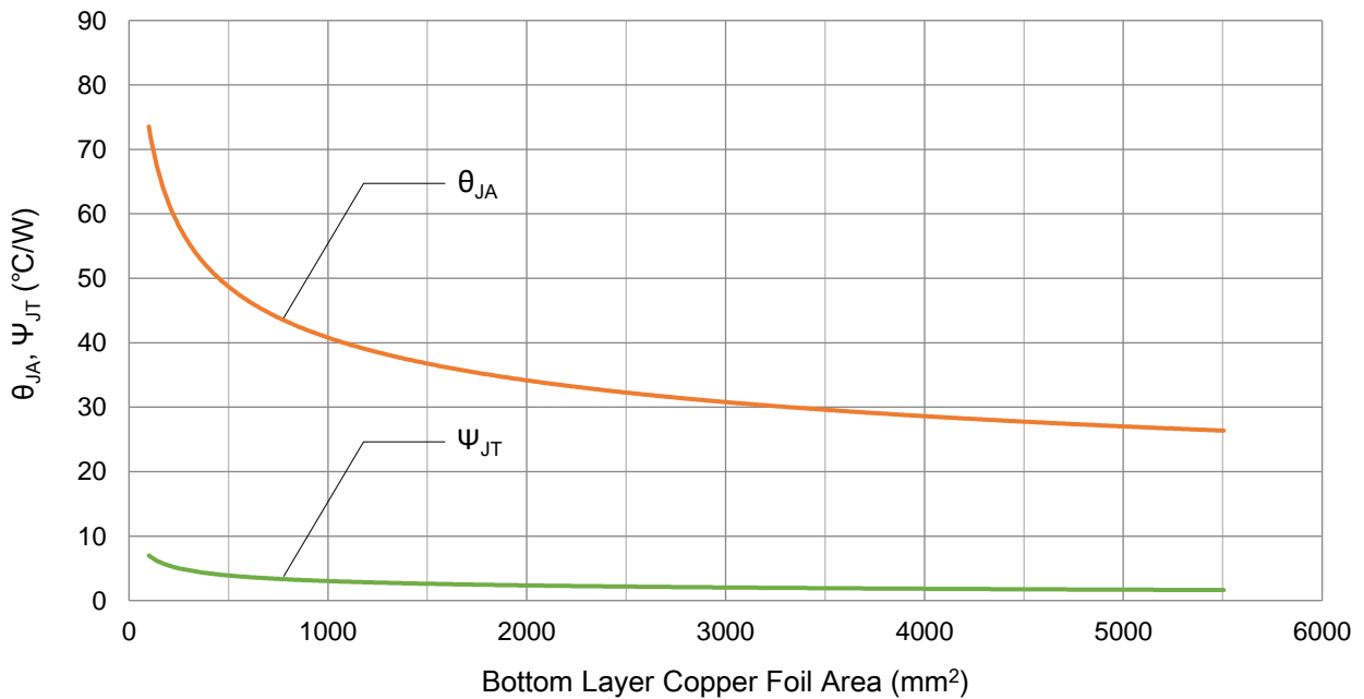
Figure 15. \theta_{JA} , \psi_{JT} vs. copper foil back surface area
