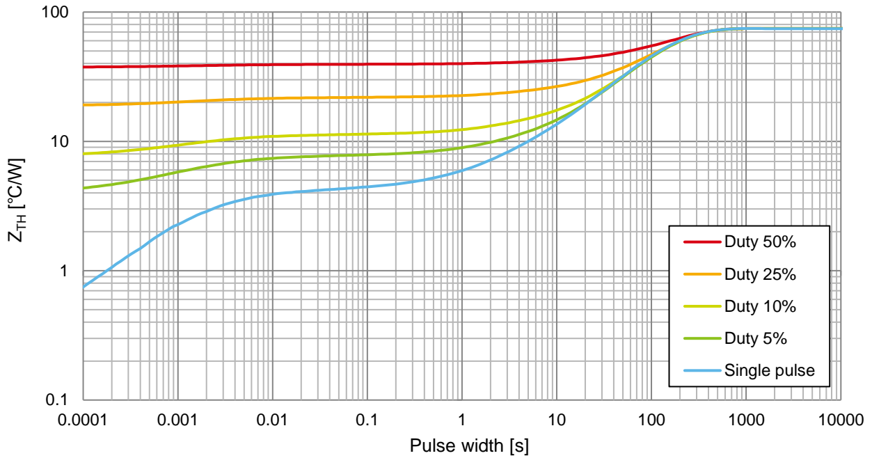
Figure 16. Transient thermal resistance, 1 layer Copper foil surface area 73.8 mm 2 (Footprint)
