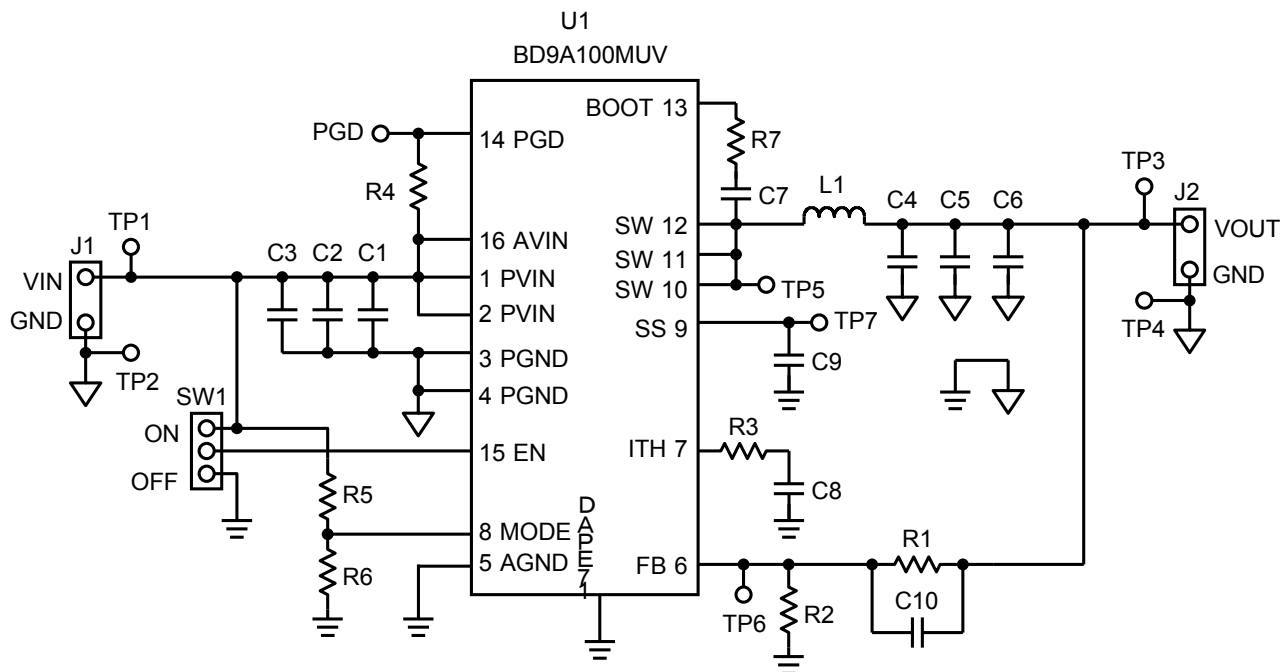
Figure 3. BD9A100MUV-EVK-001 Circuit Diagram
