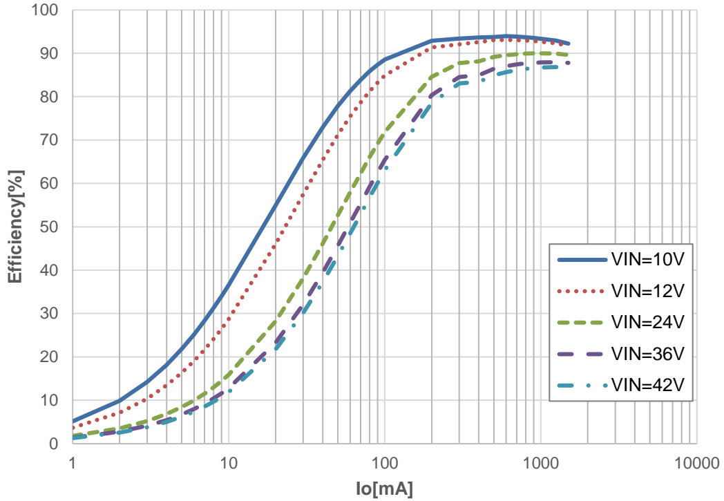
Figure 8. Efficiency vs Load Current (VOUT=5V)
