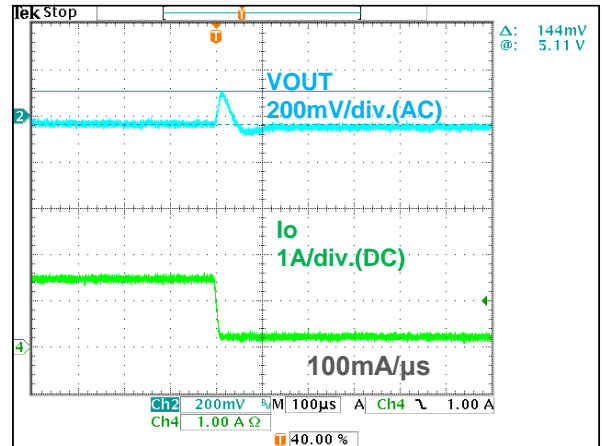
Figure 11. Transient Load Response (VIN=12V, Io=1.5A → 0.25A)
