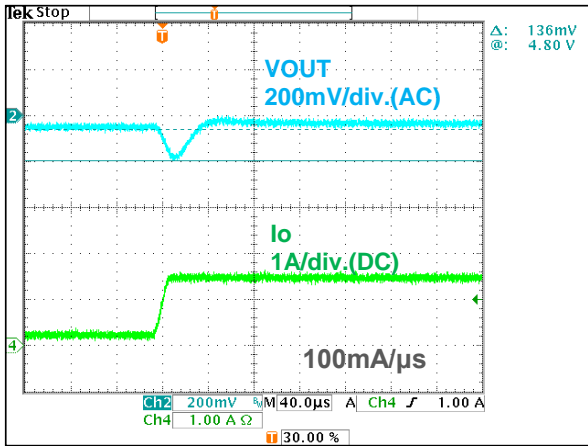
Figure 10. Transient Load Response (VIN=12V, Io=0.25A → 1.5A)
