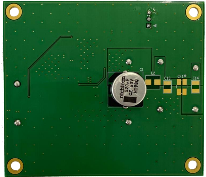
Figure 2. BD9G201EFJ-EVK-001(Bottom View)
