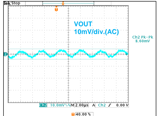
Figure 13. Output Ripple Voltage (VIN=12V, Io=1.5A)
