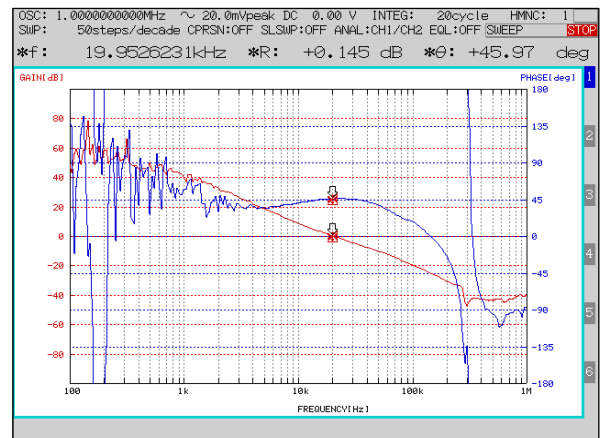
Figure 15. Frequency Characteristics (VIN=12V, Io=1.5A)
