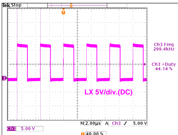
Figure 14. Switching Waveform (VIN=12V, Io=1.5A)
