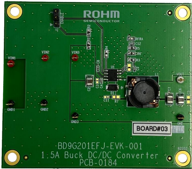
Figure 1. BD9G201EFJ-EVK-001(Top View)
