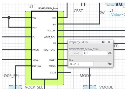
Figure 4. TSS property of BD9P205MUF-C_Tran
