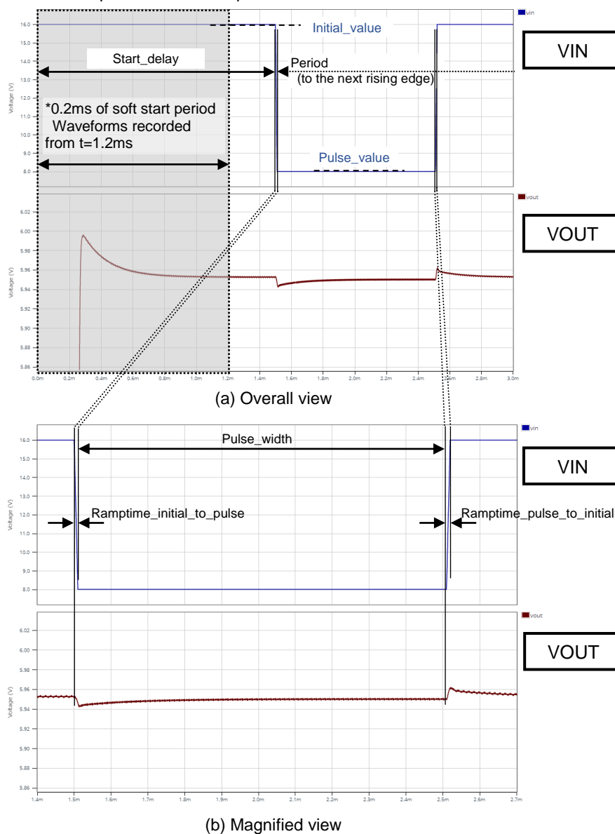
Figure 4.VIN parameters and its waveforms
