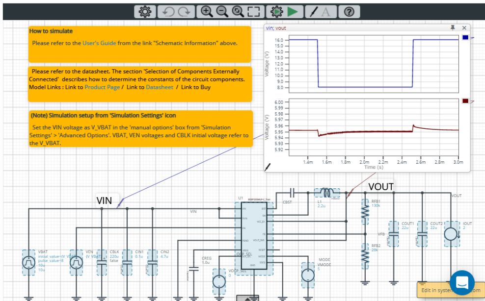
Figure 1. Simulation Schematic
