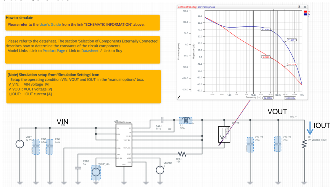
Figure 1. Simulation Circuit
