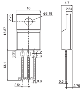
(TO-220FM)*2 (TO-220FP)
