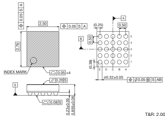
S-VFBGA25-2.76×2.50-0.50-W
