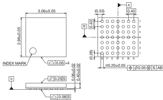
S-UFLGA48-3.06×2.96-0.40-W
