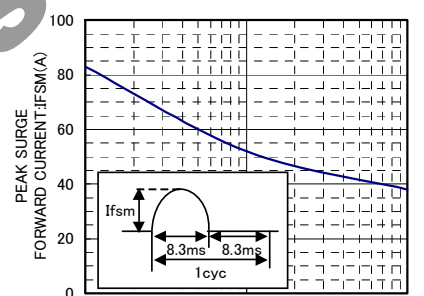
IFSM-CYCLE CHARACTERISTICS
