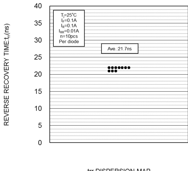
t_{tr} DISPERSION MAP
