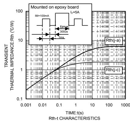
R_{\theta} - t CHARACTERISTICS
