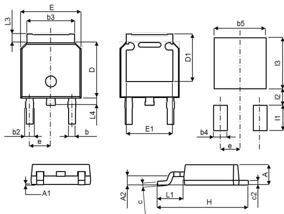
TO-252, (TO-252)
