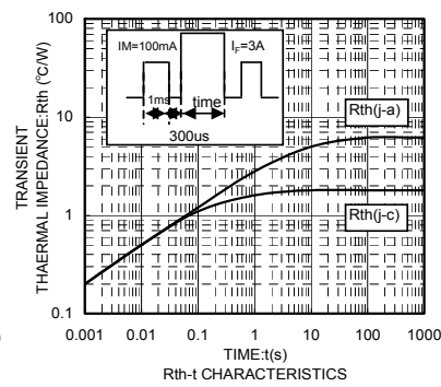
R_{th}-t CHARACTERISTICS
