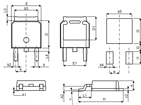
TO-252, (TO-252)
