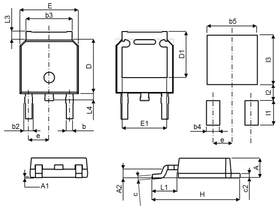
TO-252, (TO-252)
