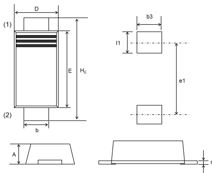
SOD-123FL, (PMDU)
