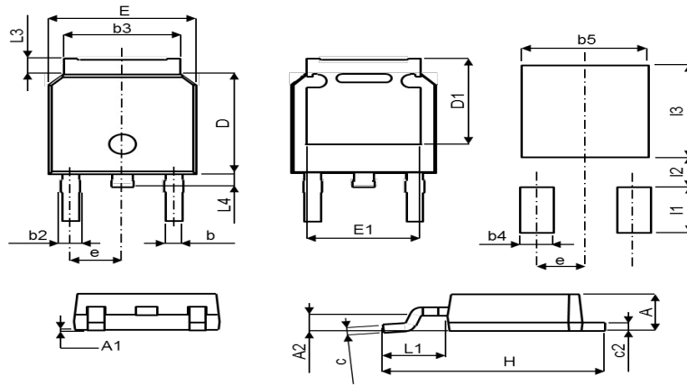
TO-252, (TO-252)
