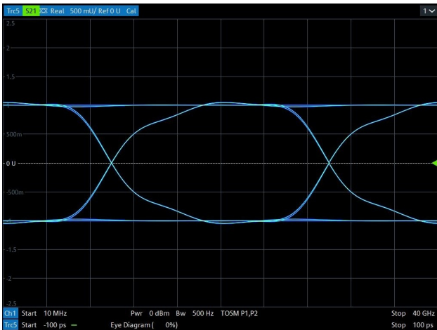
Data Rate > 10 Gbps Eye Diagram (with RES3V3BASAFH)
