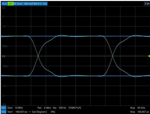
Data Rate > 6 Gbps Eye Diagram (with RES3V3BASAFH)
