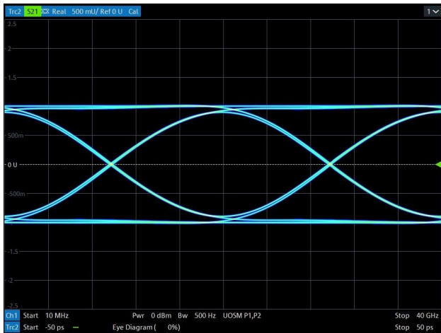
Data Rate > 20 Gbps Eye Diagram (with RES3V3UCED)
