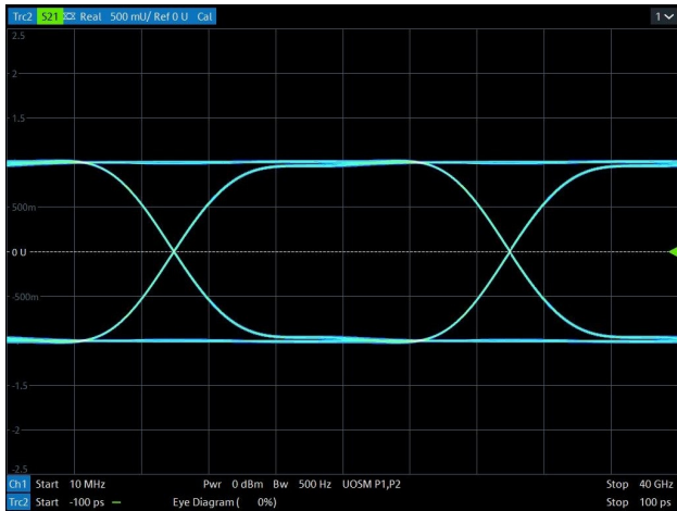
Data Rate > 10 Gbps Eye Diagram (with RES3V3UCED)
