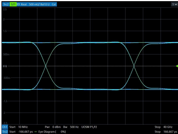
Data Rate > 6 Gbps Eye Diagram (with RES3V3UCED)
