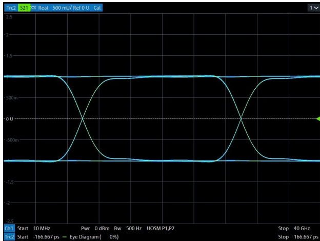
Data Rate > 6 Gbps Eye Diagram (with RES3V6UCED)
