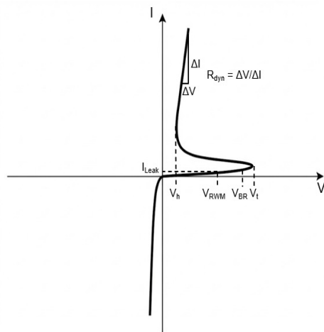
I-V characteristics for a unidirectional ESD protection diode
