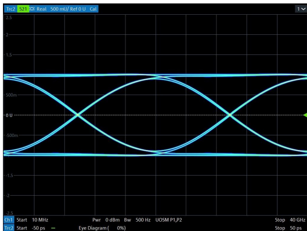
Data Rate > 20 Gbps Eye Diagram (with RES3V6UCED)
