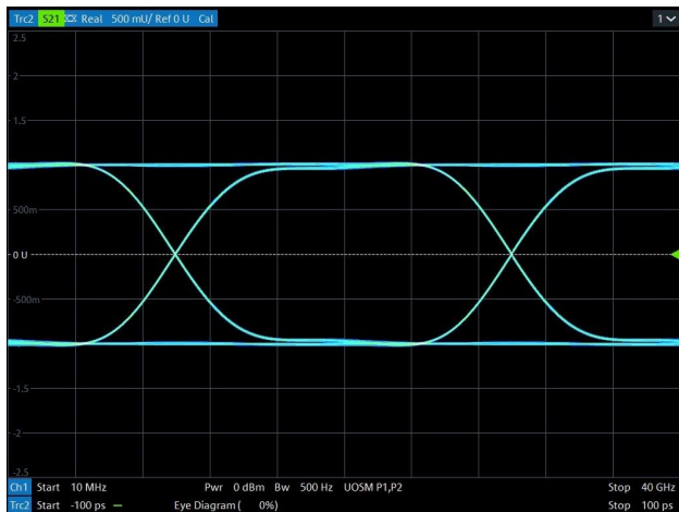
Data Rate > 10 Gbps Eye Diagram (with RES3V6UCED)
