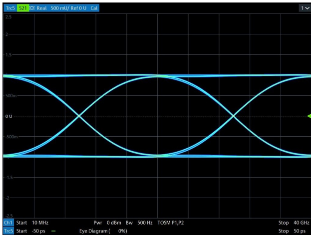
Data Rate > 20 Gbps Eye Diagram (with RES5V0BAED)
