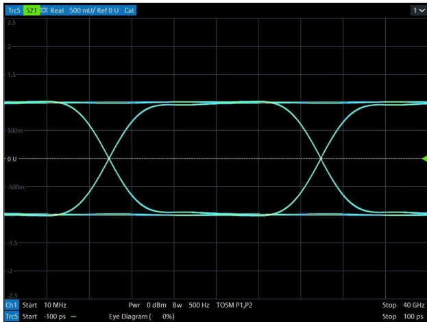
Data Rate > 10 Gbps Eye Diagram (with RES5V0BAED)
