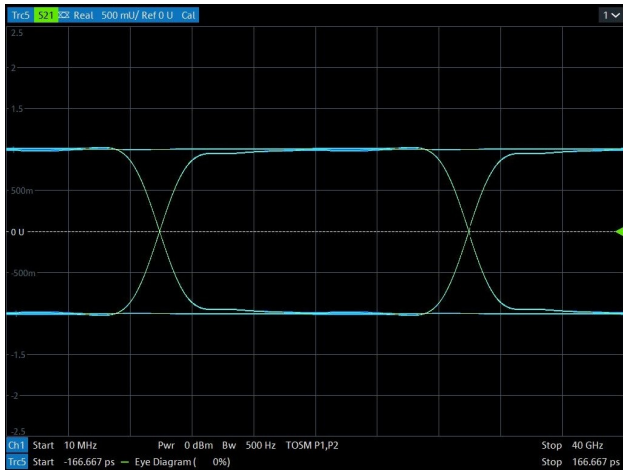
Data Rate > 6 Gbps Eye Diagram (with RES5V0BAED)
