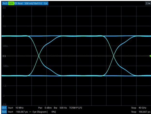
Data Rate > 6 Gbps Eye Diagram (with RES5V0BASAFH)
