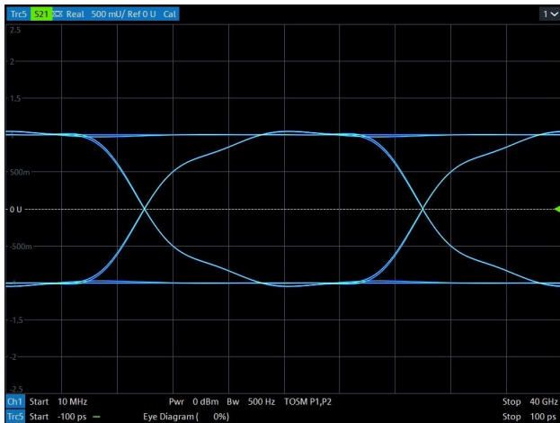
Data Rate > 10 Gbps Eye Diagram (with RES5V0BASAFH)
