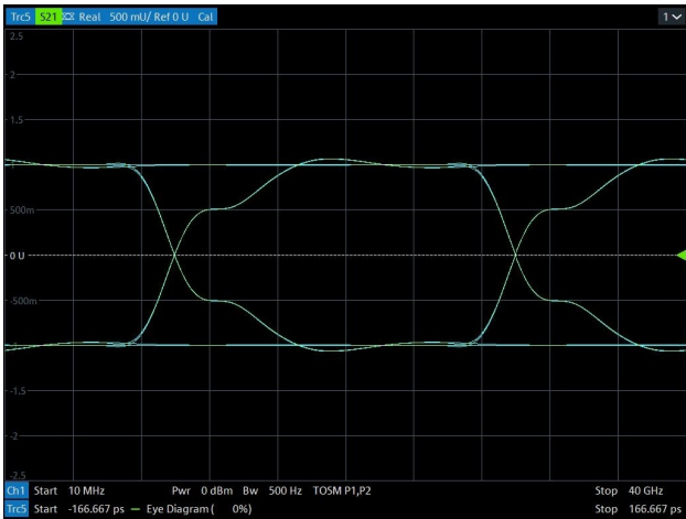
Data Rate > 6 Gbps Eye Diagram (with RES5V0UASAFH)
