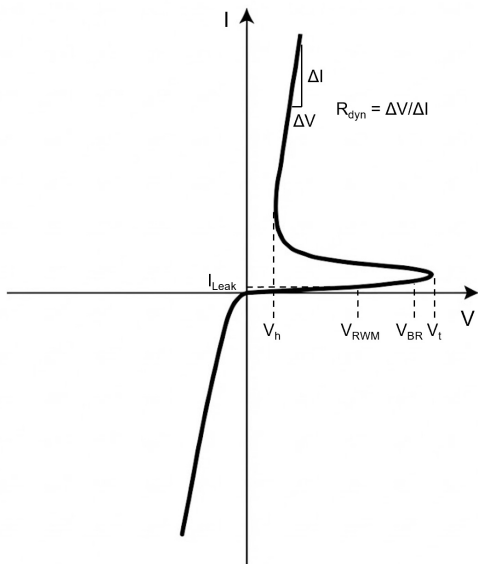
I-V characteristics for a unidirectional ESD protection diode
