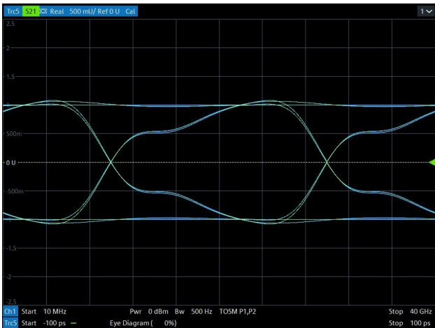
Data Rate > 10 Gbps Eye Diagram (with RES5V0UASAFH)
