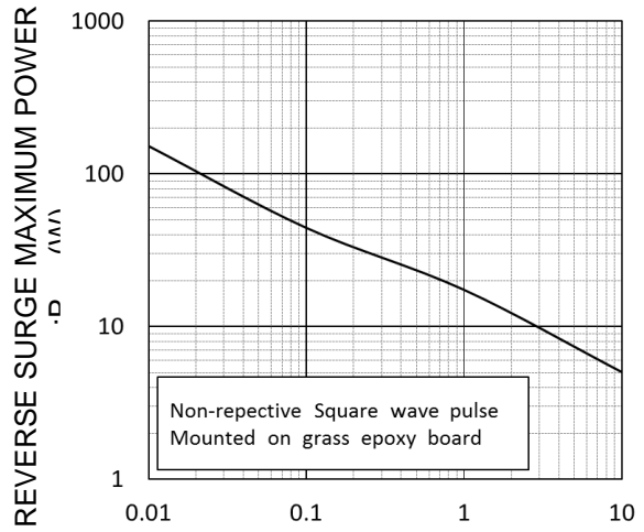
PULSE TIME: t (ms) P_{RSM} - t CHARACTERISTICS
