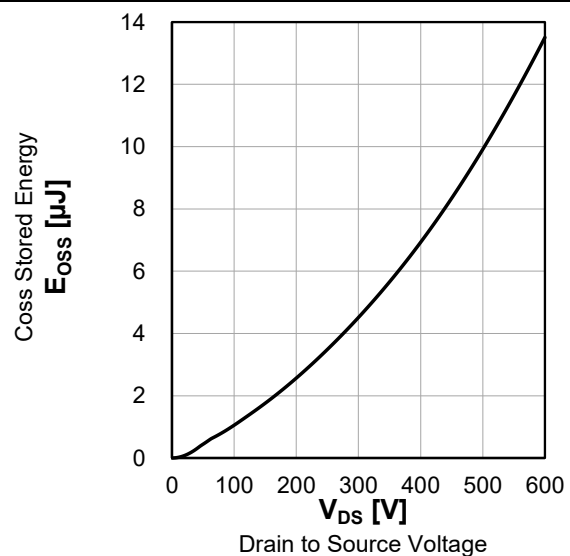
Fig.16 Typ. Coss Stored Energy
