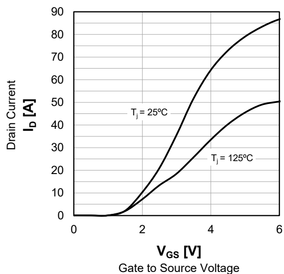
Fig.8 Typ. Transfer Characteristics
