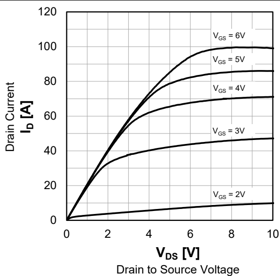
Fig.5 Typ. Output Characteristics
