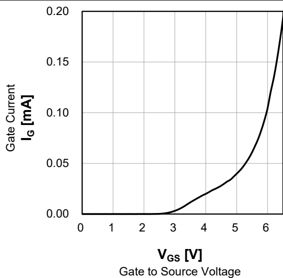
Fig.9 Gate to Source Leakage Characteristics
