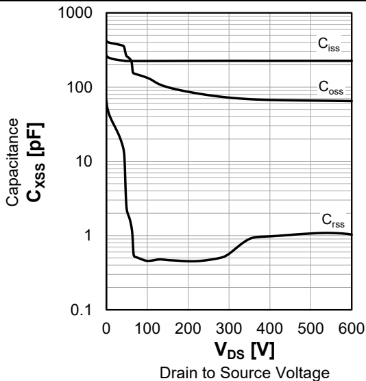
Fig.15 Typ. Capacitance
