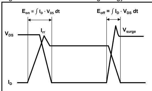
Fig.21 Waveforms for Switching Energy Loss
