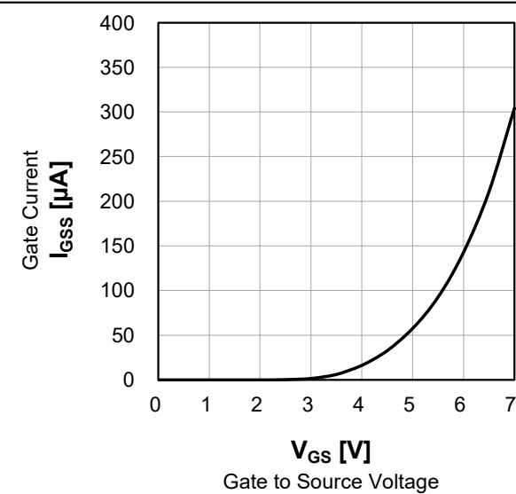
Fig.9 Gate to Source Leakage Characteristics
