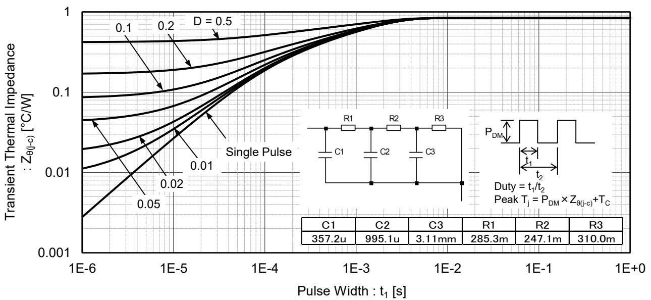
Fig.26 Typical Diode Transient Thermal Impedance
