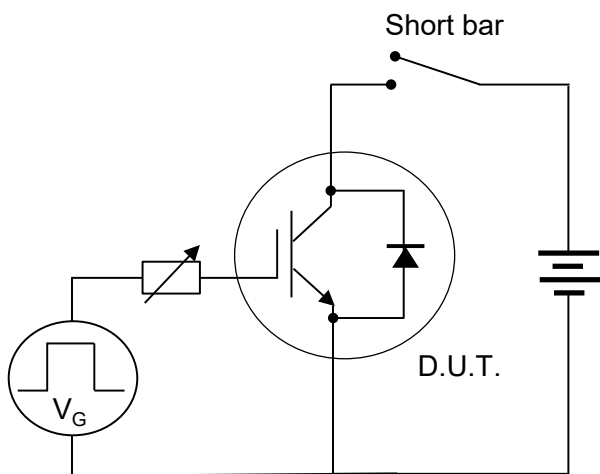
Fig.30 Short Circuit
