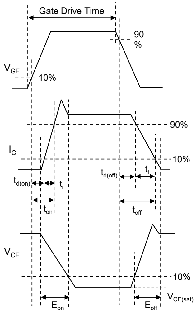
Fig.29 Inductive Load Waveform
