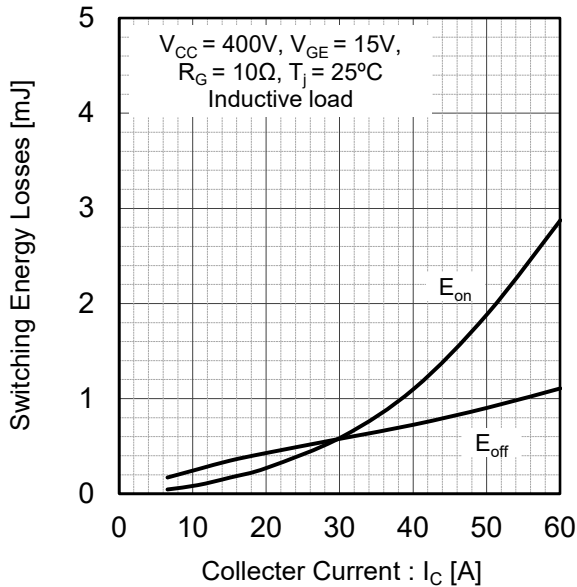
Fig.15 Typical Switching Energy Losses vs. Collector Current
