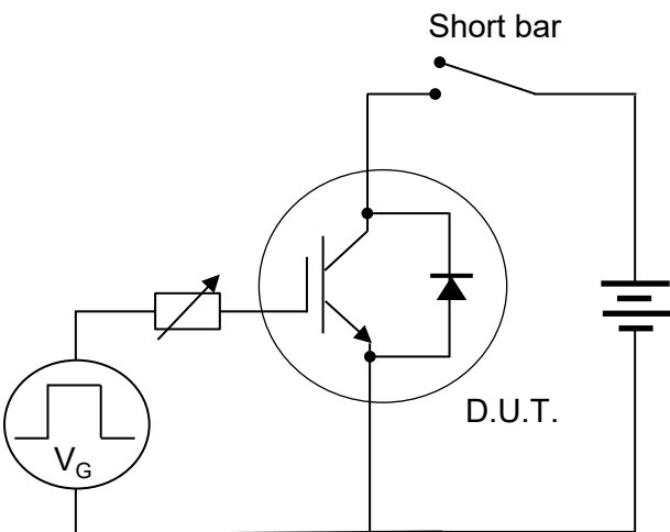
Fig.30 Short Circuit
