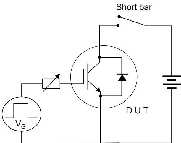
Fig.30 Short Circuit
