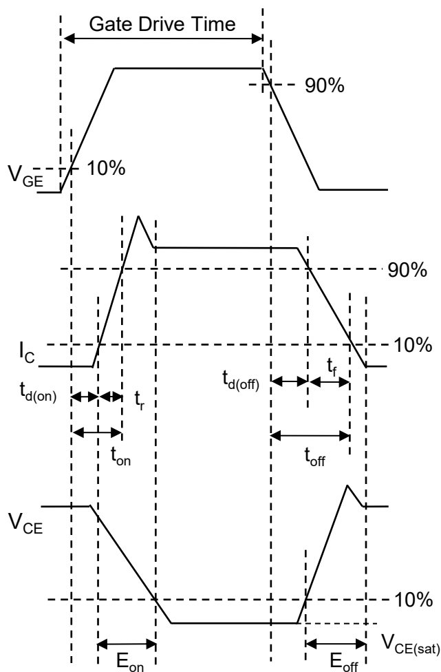
Fig.29 Inductive Load Waveform
