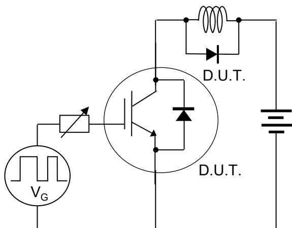
Fig.27 Inductive Load Circuit
