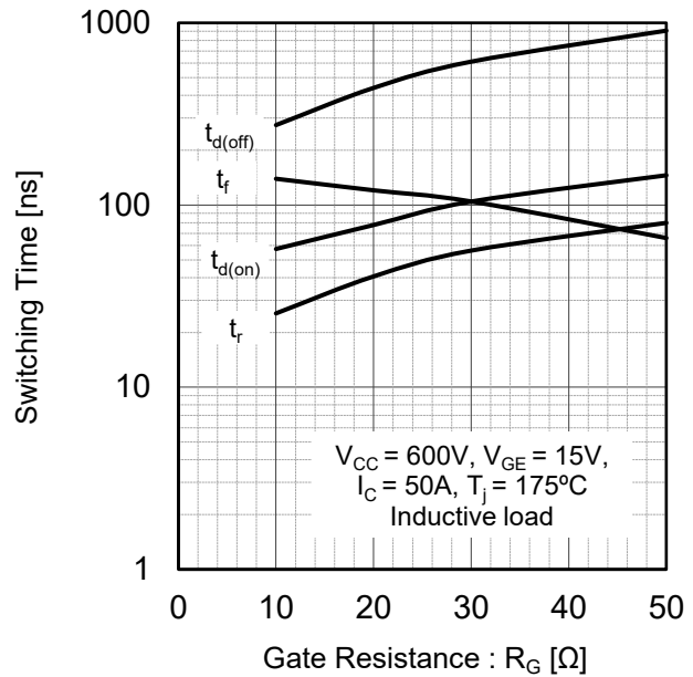
Fig.18 Typical Switching Time vs. Gate Resistance
