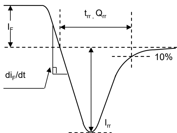
Fig.28 Diode Reverse Recovery Waveform
