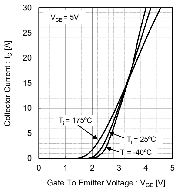
Fig.7 Typical Transfer Characteristics
