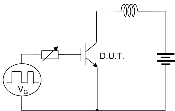
Fig.19 Self Clamped Inductive Switching Circuit
