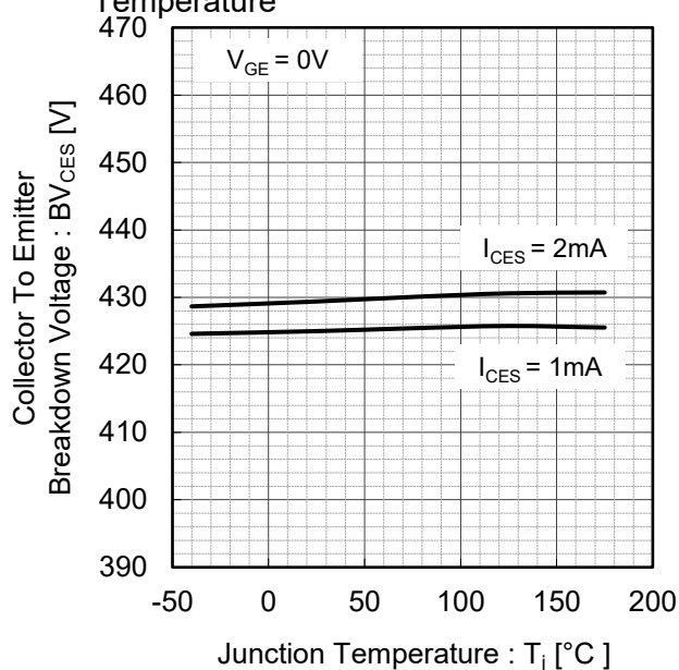
Fig.10 Typical Collector To Emitter Breakdown Voltage vs. Junction Temperature
