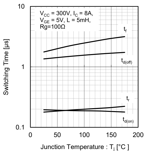
Fig.14 Typical Switching Time vs. Junction Temperature
