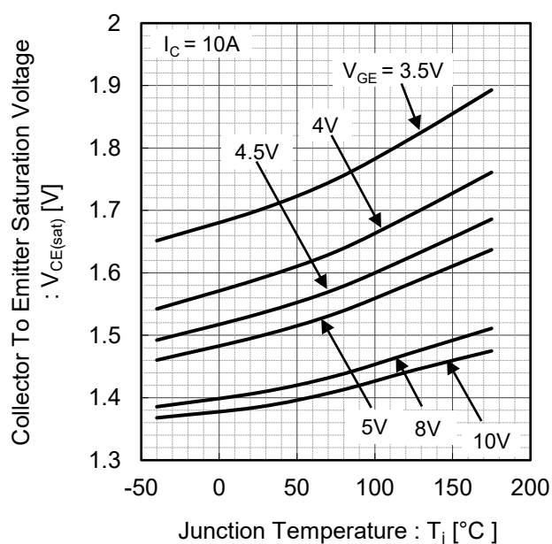
Fig.5 Typical Collector To Emitter Saturation Voltage vs. Junction Temperature
