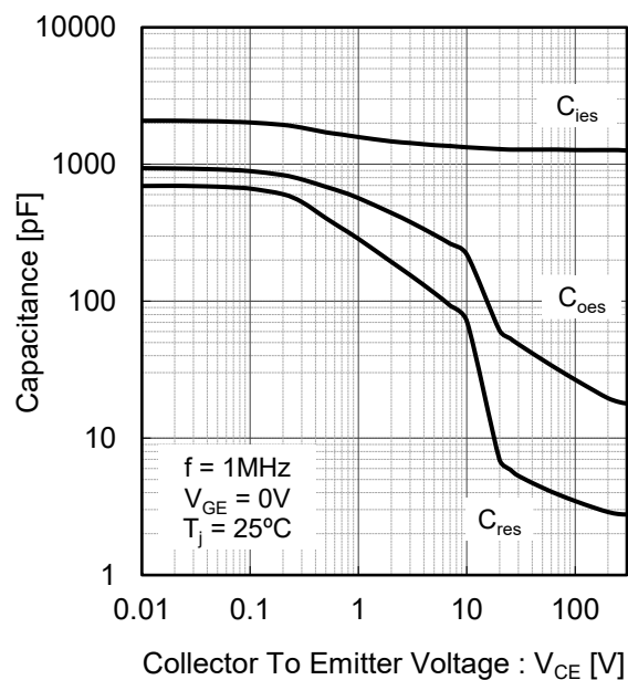
Fig.13 Typical Capacitance vs. Collector To Emitter Voltage
