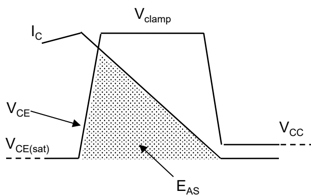
Fig.20 Self Clamped Inductive Switching Waveform
