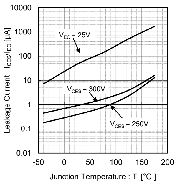
Fig.9 Typical Leakage Current vs. Junction Temperature
