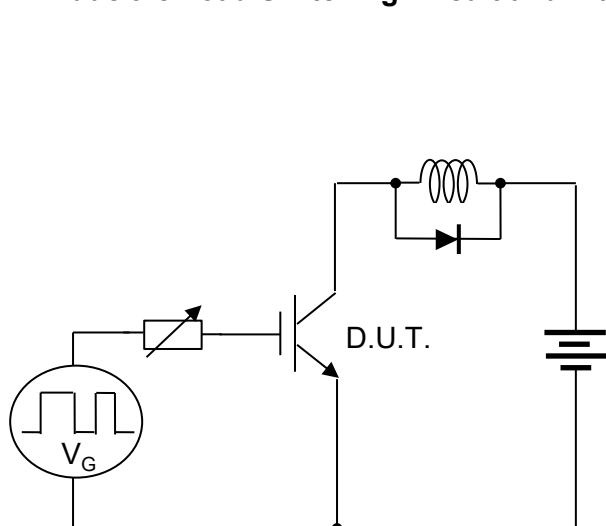
Fig.17 Inductive Load Switching Circuit
