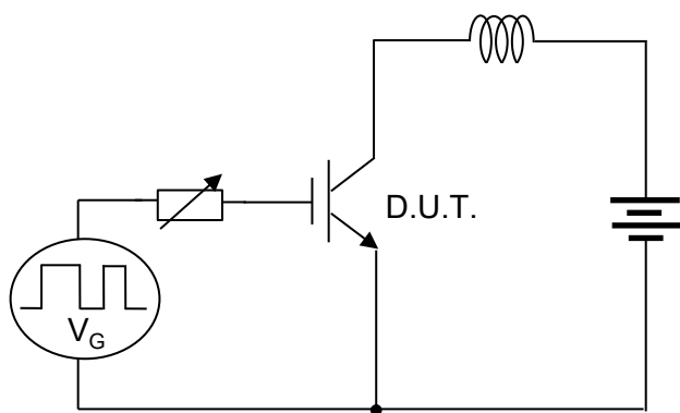
Fig.19 Self Clamped Inductive Switching Circuit
