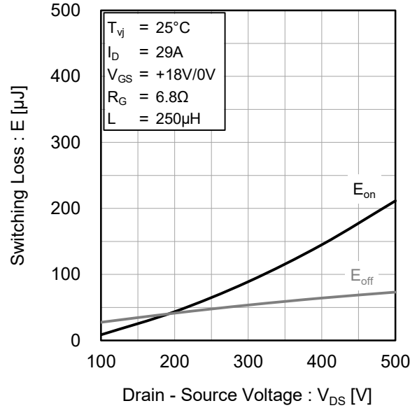
Fig.21 Typical Switching Loss vs. Drain - Source Voltage
