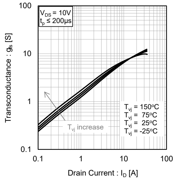
Fig.12 Transconductance vs. Drain Current
